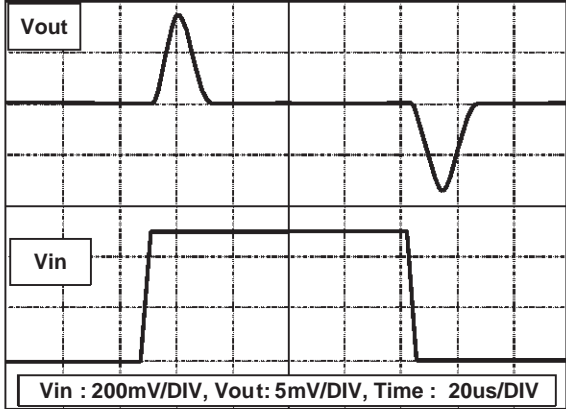
V CC = 4.75 to 5.25V, I OUT = 0.1A, C O = 10μF (ESR=1Ω at 1KHz)
