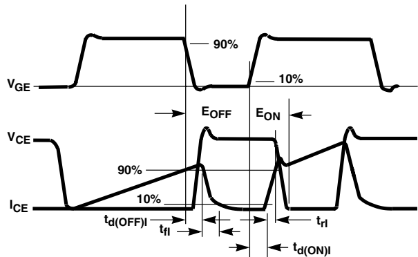
FIGURE 17. SWITCHING TEST WAVEFORMS
