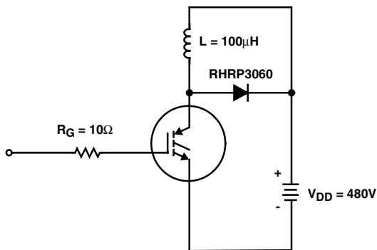
FIGURE 16. INDUCTIVE SWITCHING TEST CIRCUIT
